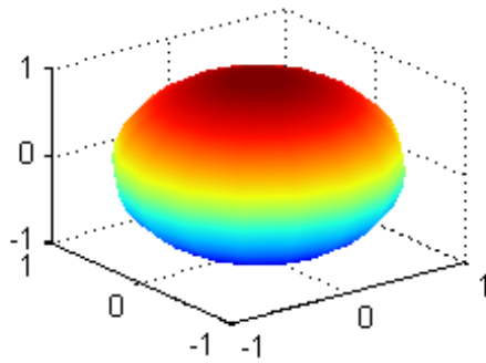
Interpolated Shading
