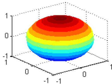
Flat Shading
